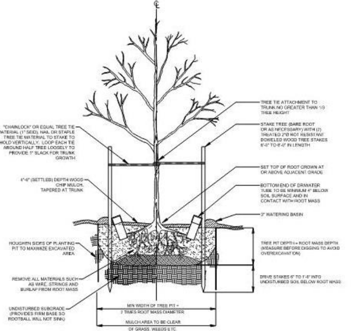
TYPICAL TREE PLANTING DETAIL R15
