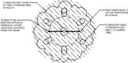
TYPICAL TREE PLANTING LAYOUT DETAIL R15
